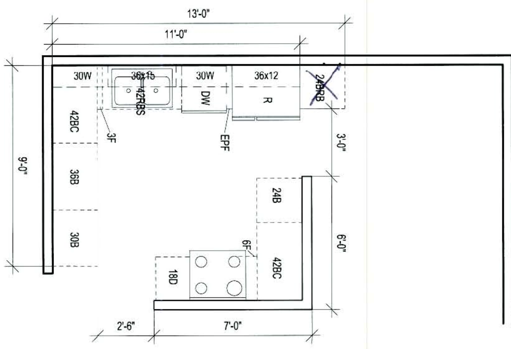
OPTION 2 - WITH PANTRY
